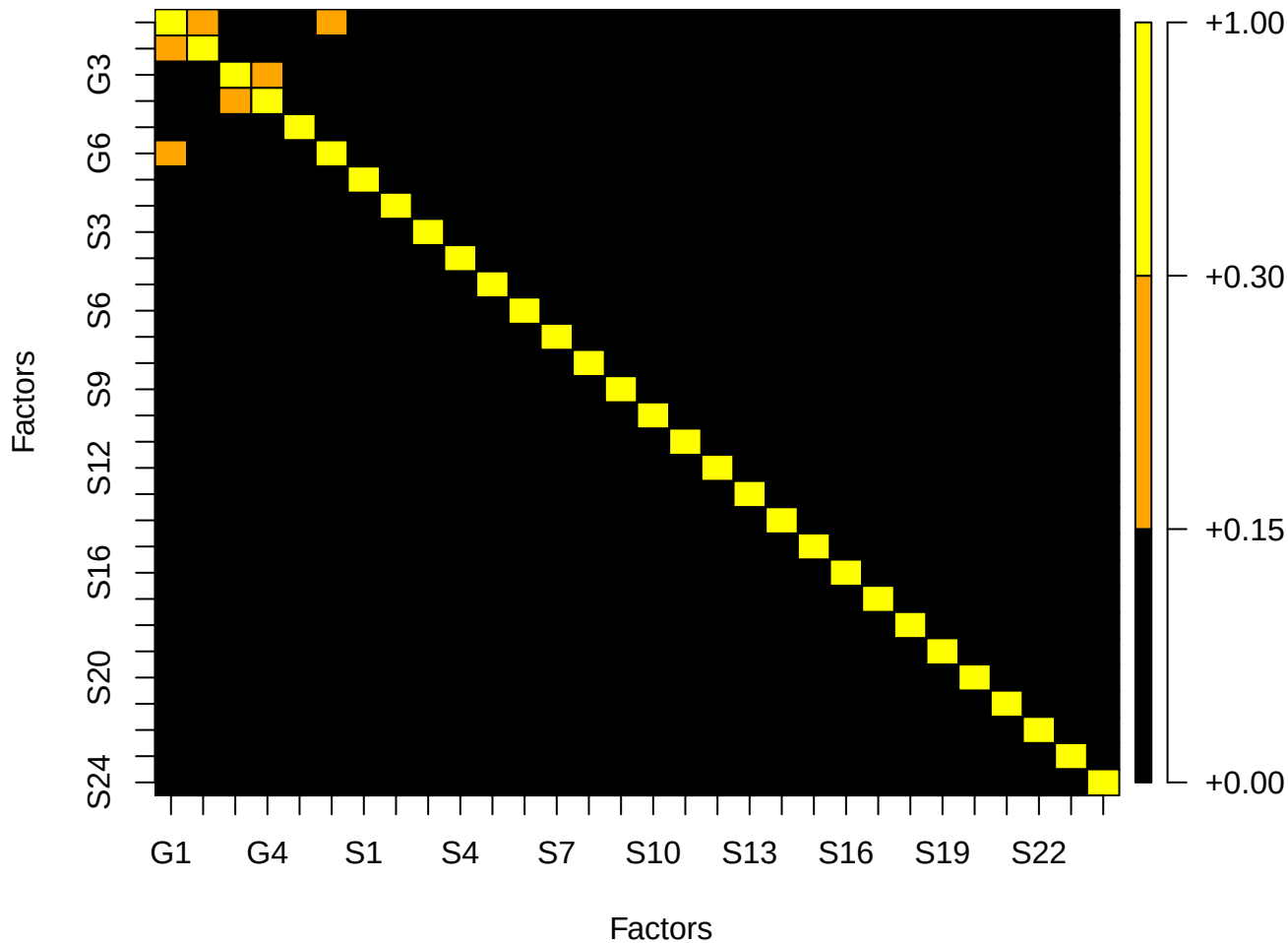
Absolute value of factor correlations (geomin + target)
